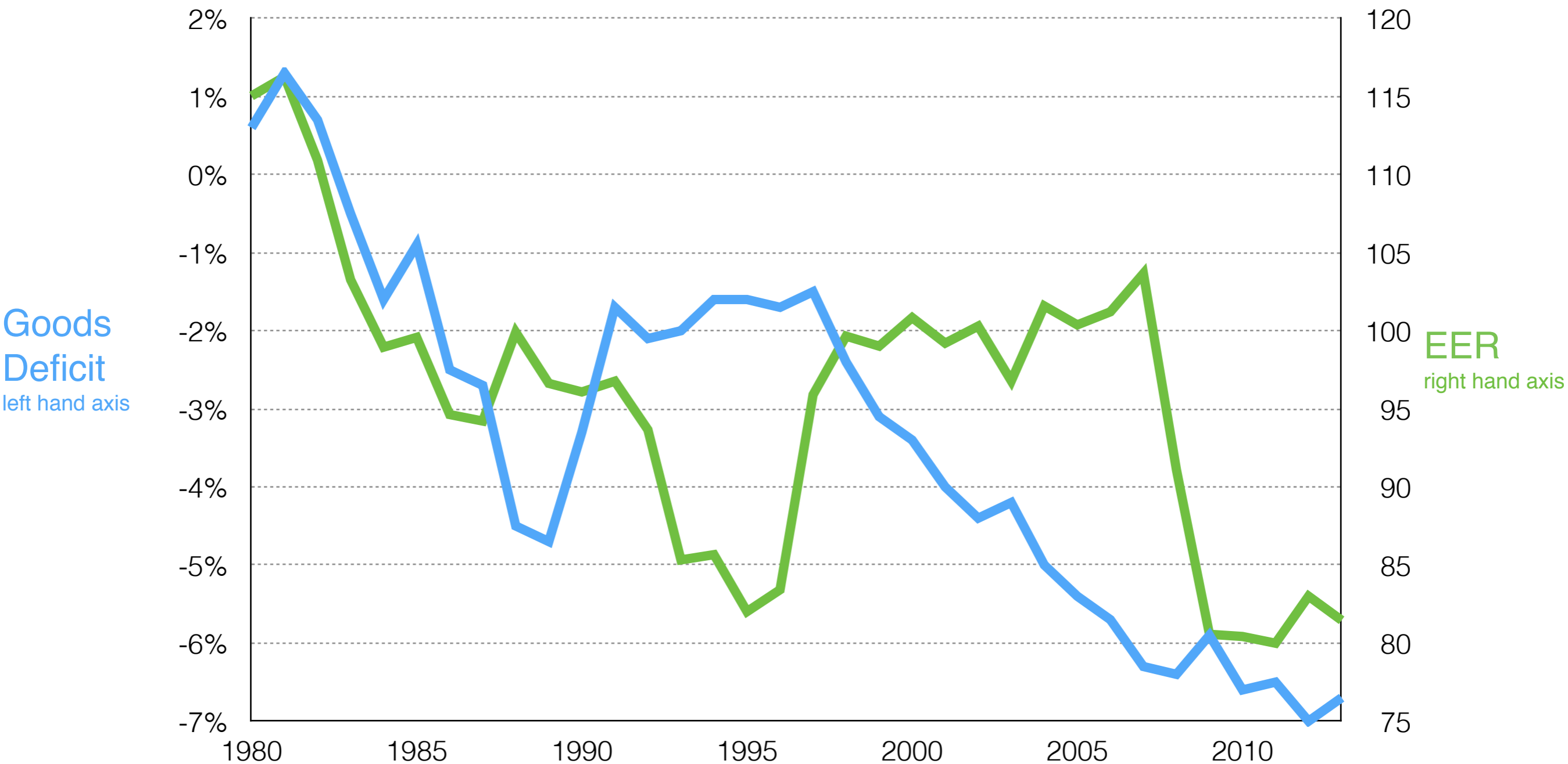
Chart 17 Trade in Goods Deficit and Sterling EER.
